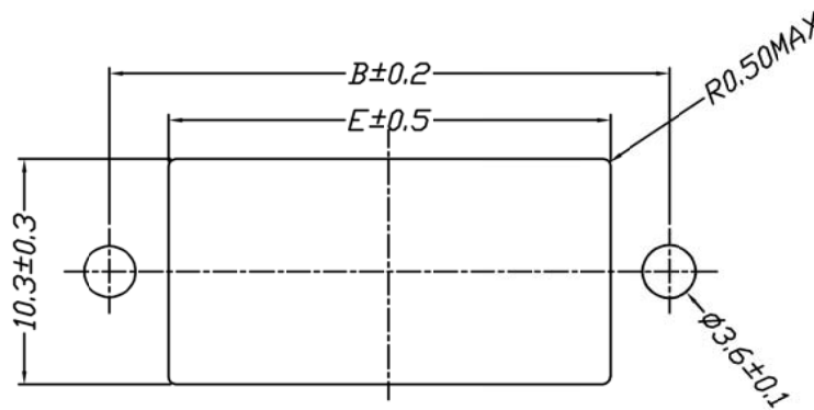
RECOMMENDED PANEL LAYOUT
