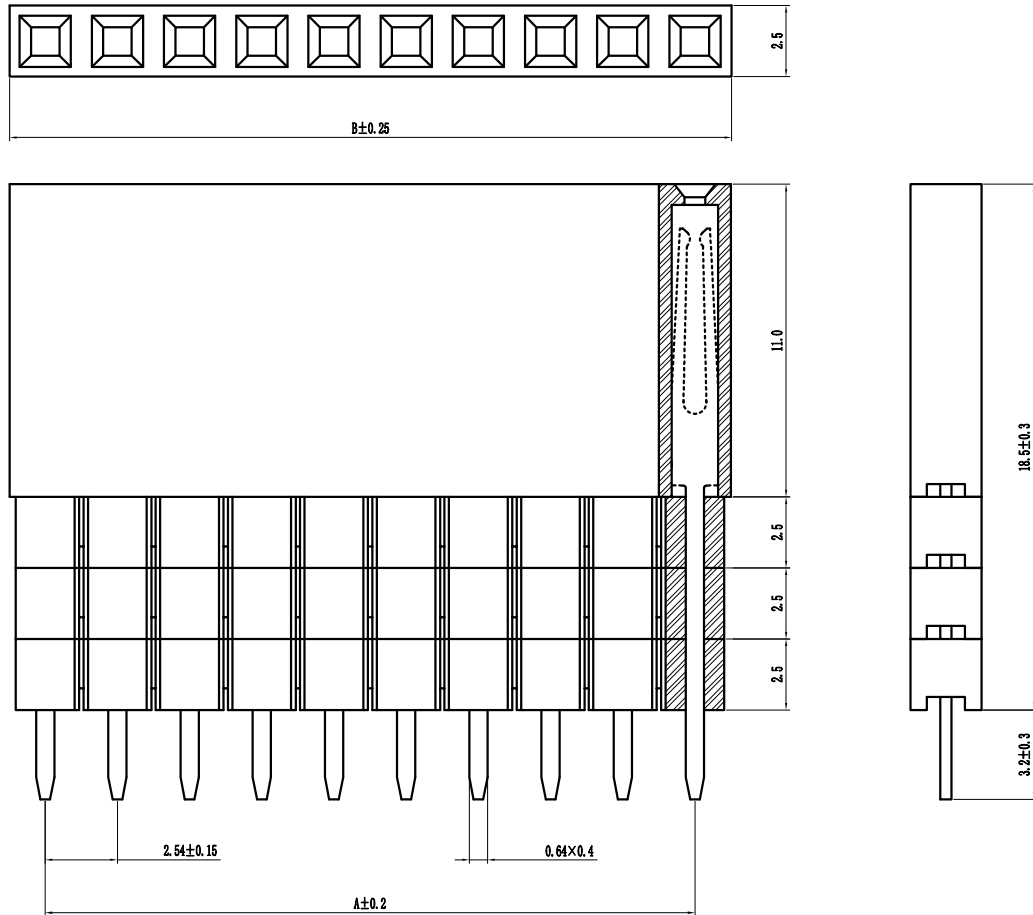
PCB LAYOUT
