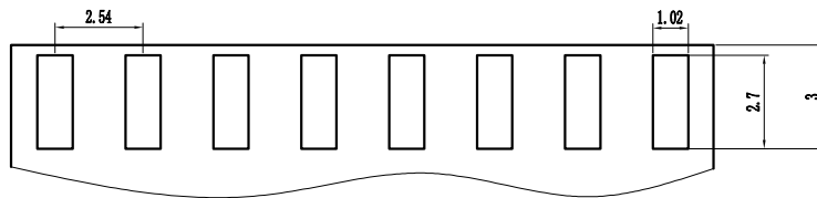
PCB LAYOUT t=1.0/1.5/2.0
