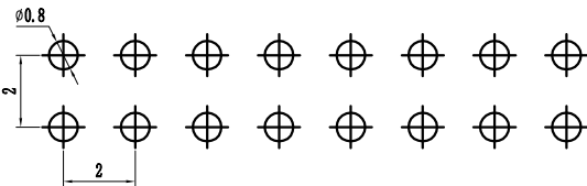
PCB LAYOUT
