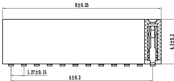
PCB LAYOUT
