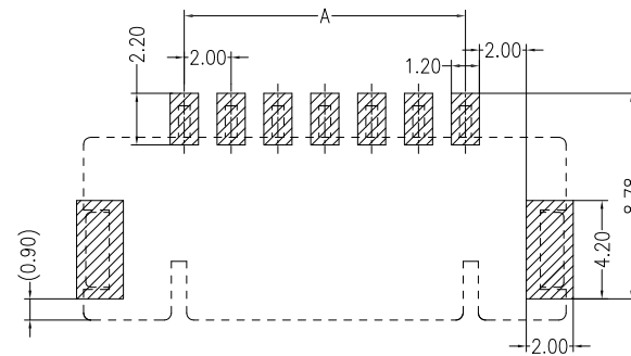
PCB LAYOUT(Tolerance:±0.05)
