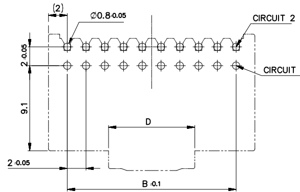
PCB LAYOUT
