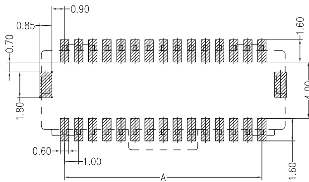
PCB LAYOUT(Tolerance:±0.05)
